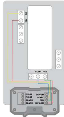
4028531 QUEST DEH 3000R CONTROL WIRING DIAGRAM
